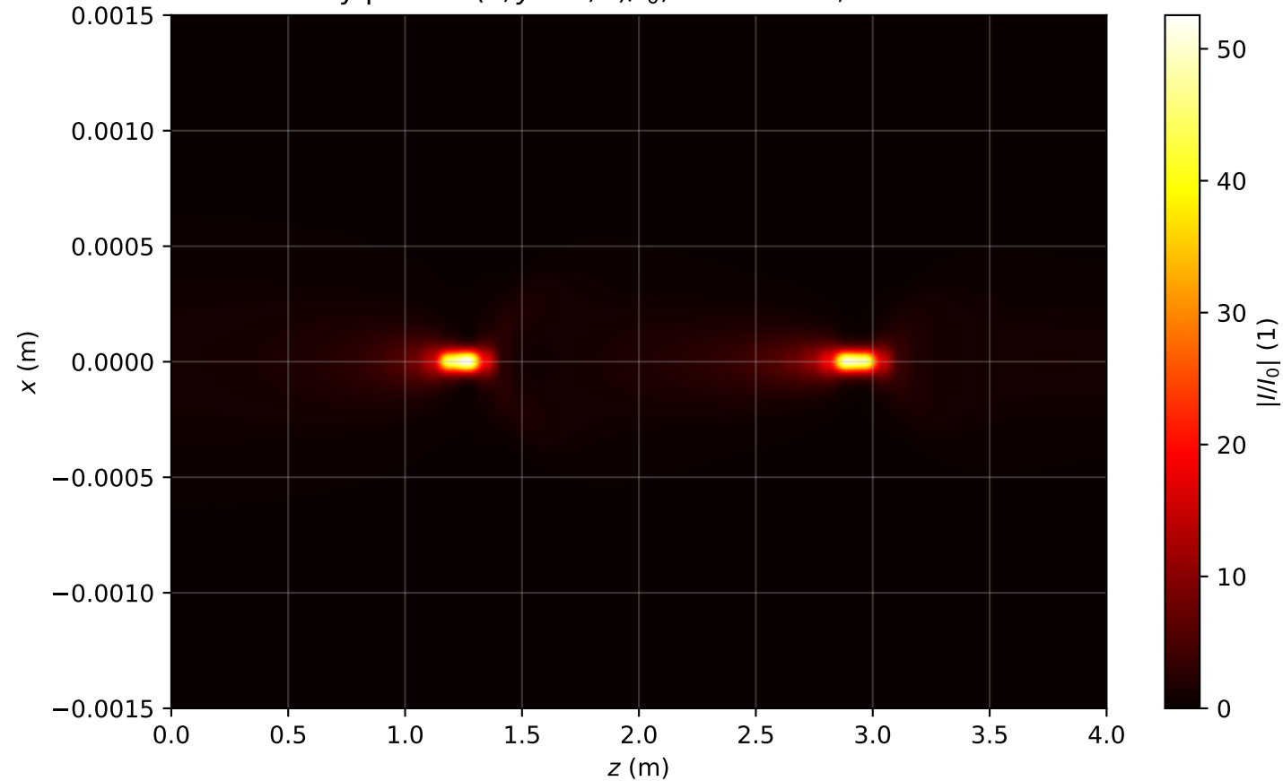
Intensity profile I(x, y = 0, z)/I_0 , P_{in}=1.9P_{cr} , artificial time
